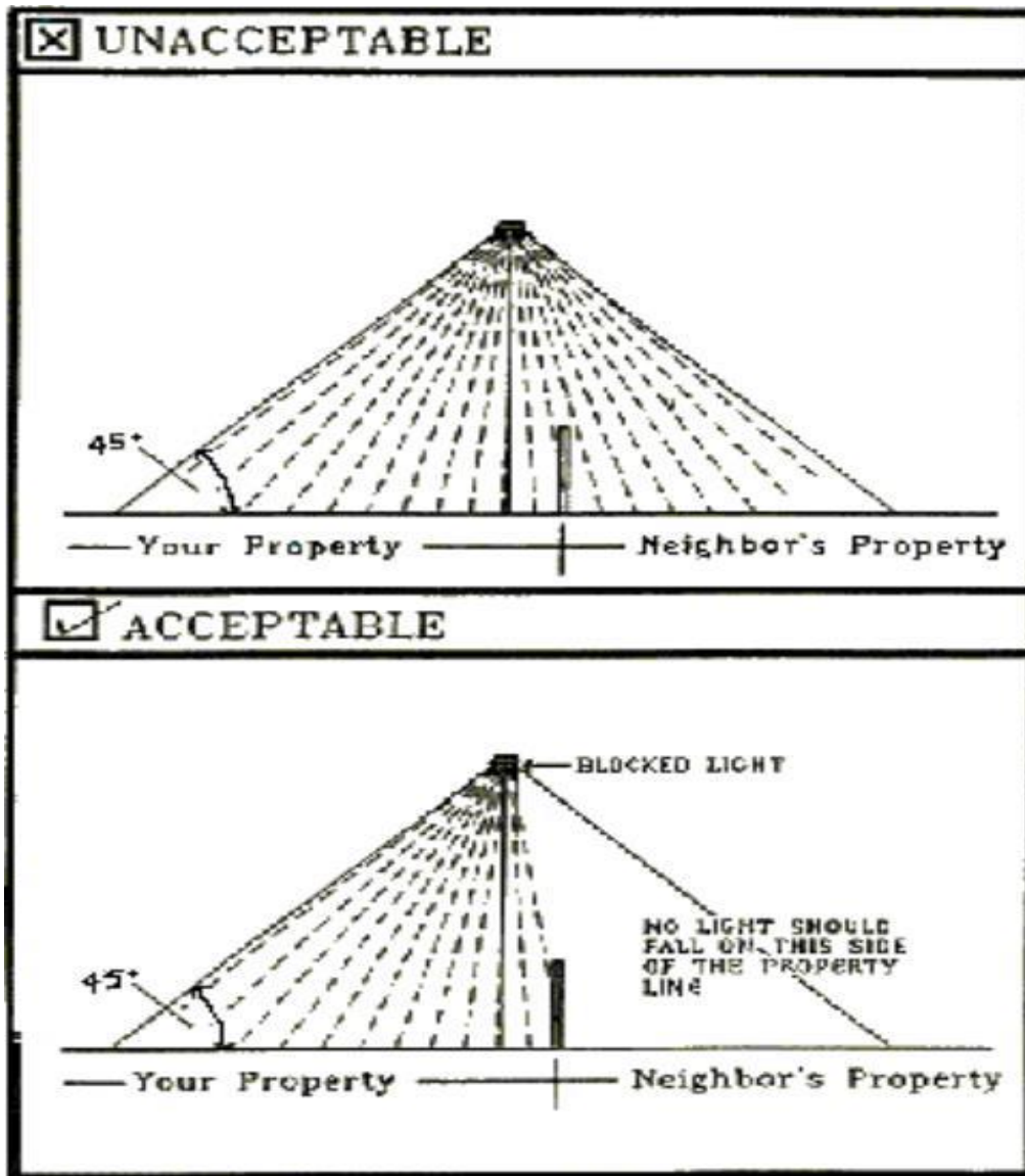
Figure 3: Outdoor Lighting Fixtures—Street and Lot Light Cut-Off at Property Line
