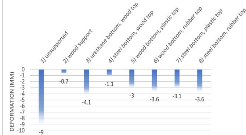
Figure 2-5. A) Set-up for static compression testing. B) Measured results from compression testing.
