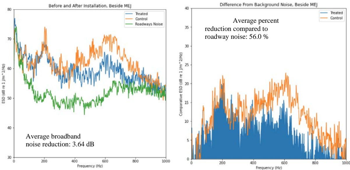
Figure 4-7. Comparison between control and initial results directly beside the MEJ.
