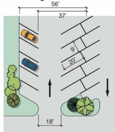
60° Parking
