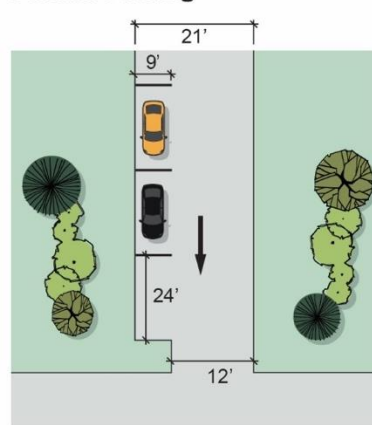
Parallel Parking
