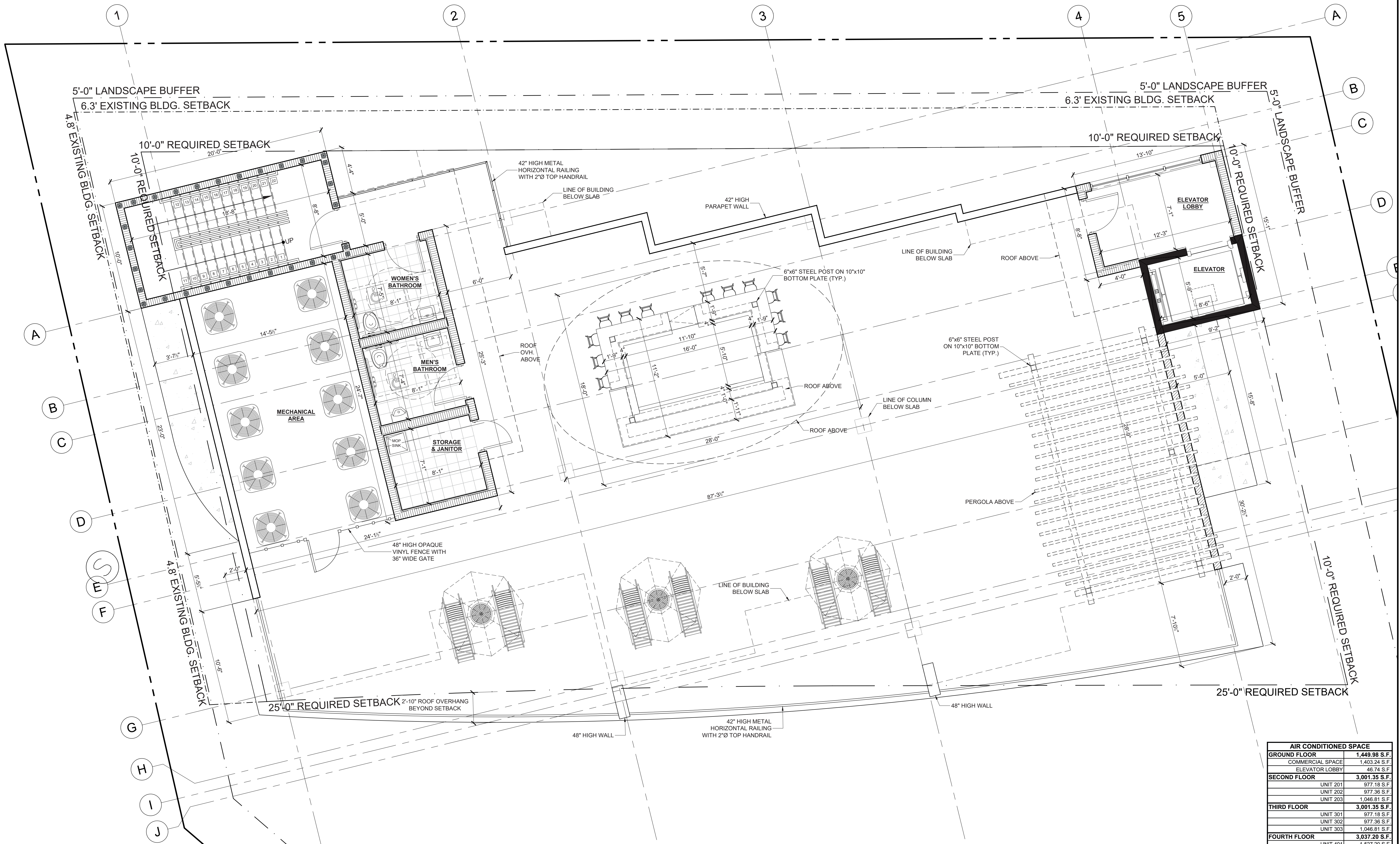
1 ROOF DECK PLAN SCALE: 1/4" = 1'-0" NORTH
