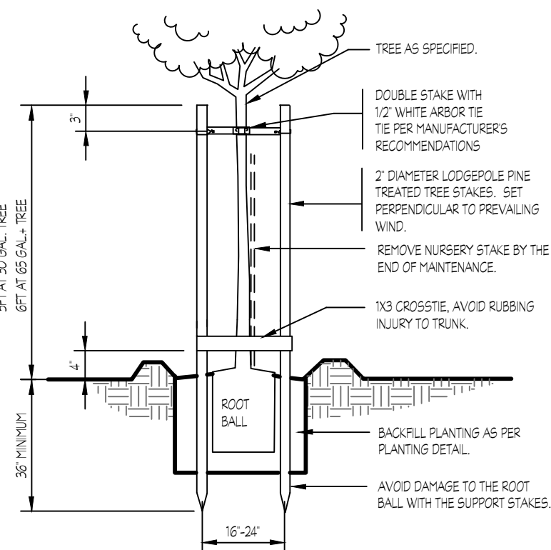
STAKING DETAIL
