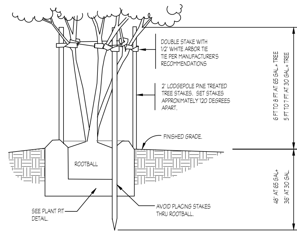
STAKING DETAIL
