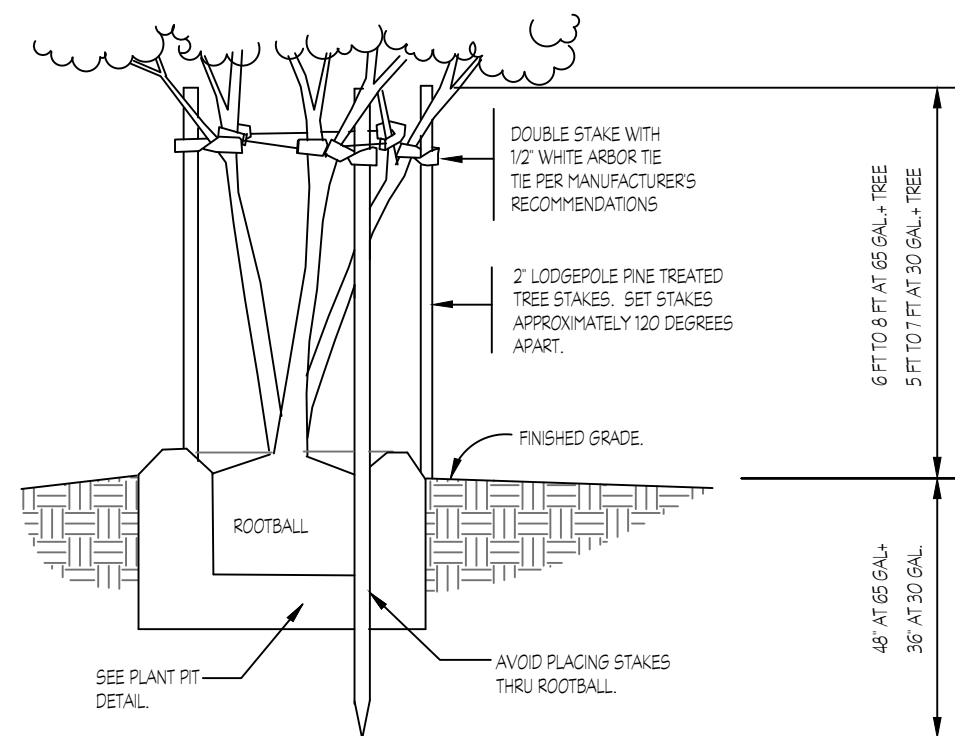
STAKING DETAIL
