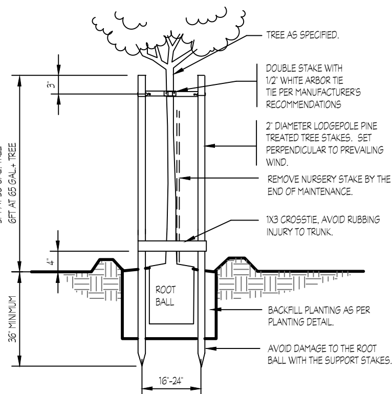
STAKING DETAIL
