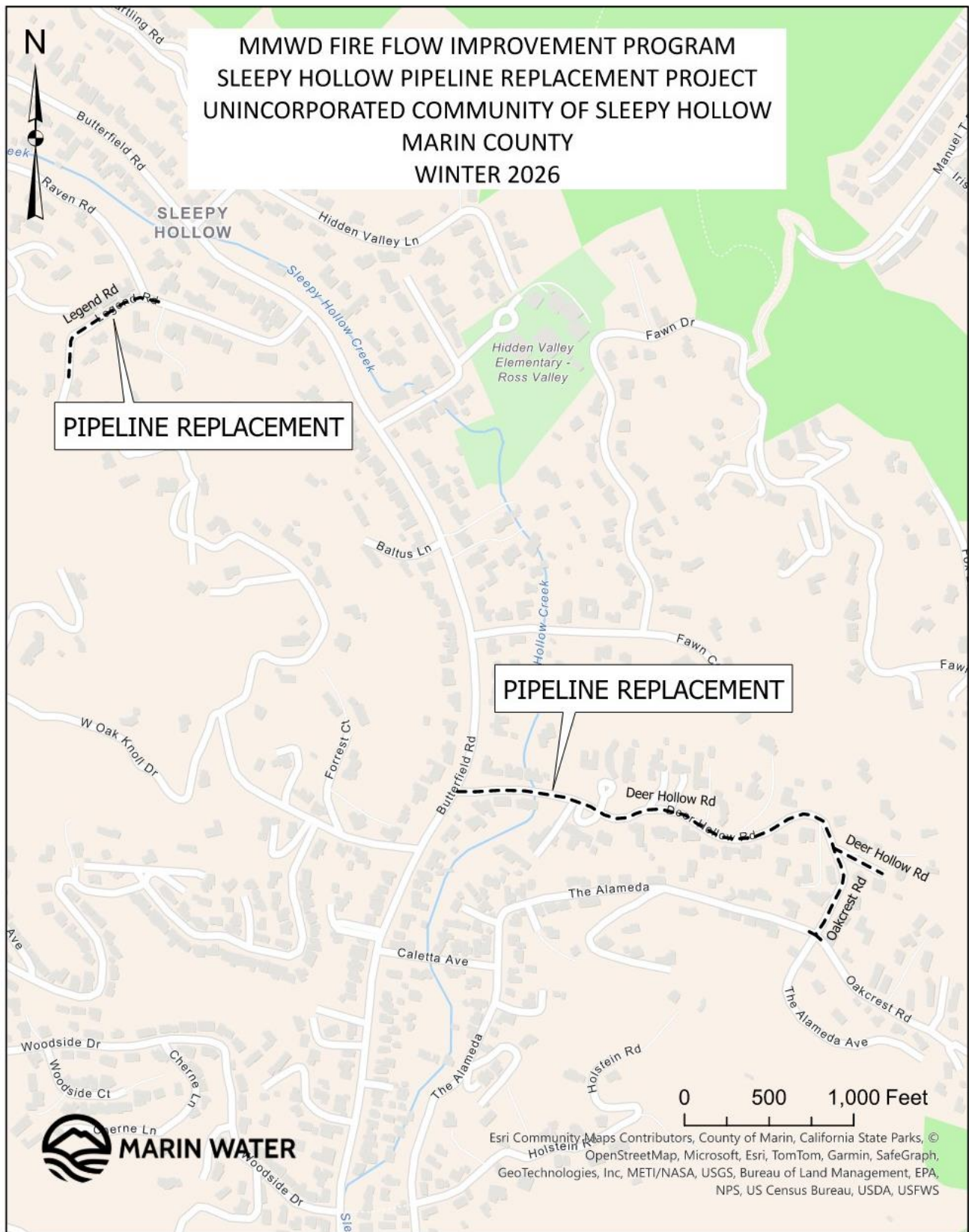
Figure 1. Site Map for the Fire Flow Improvement Program – Sleepy Hollow Pipeline Replacement Project.
