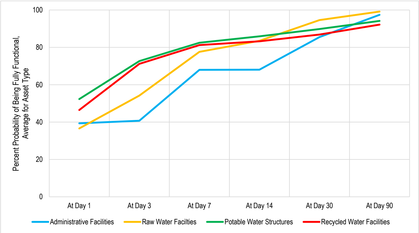
Figure 8-11. Average Probability of Full Functionality After San Gregorio M7.44 Event
