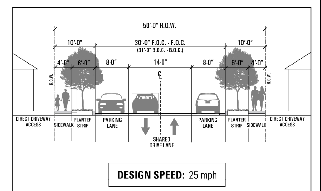
PRIMARY COLLECTOR (WITH SF-1 FRONTAGE)
