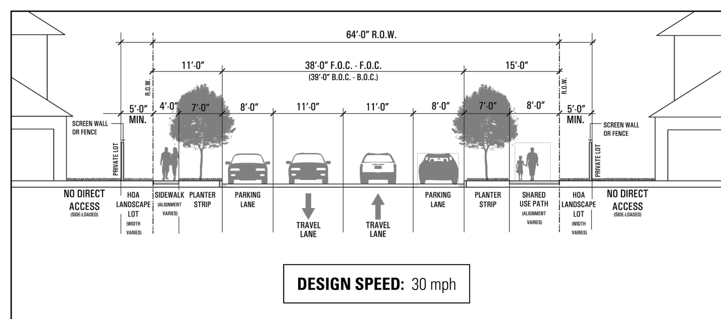
PRIMARY COLLECTOR (WITH NO SF-1 FRONTAGE)
