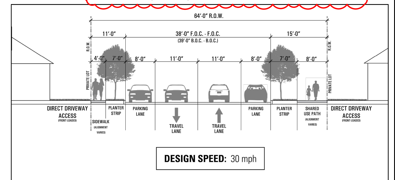
PRIMARY COLLECTOR (WITH SF-1 FRONTAGE)
