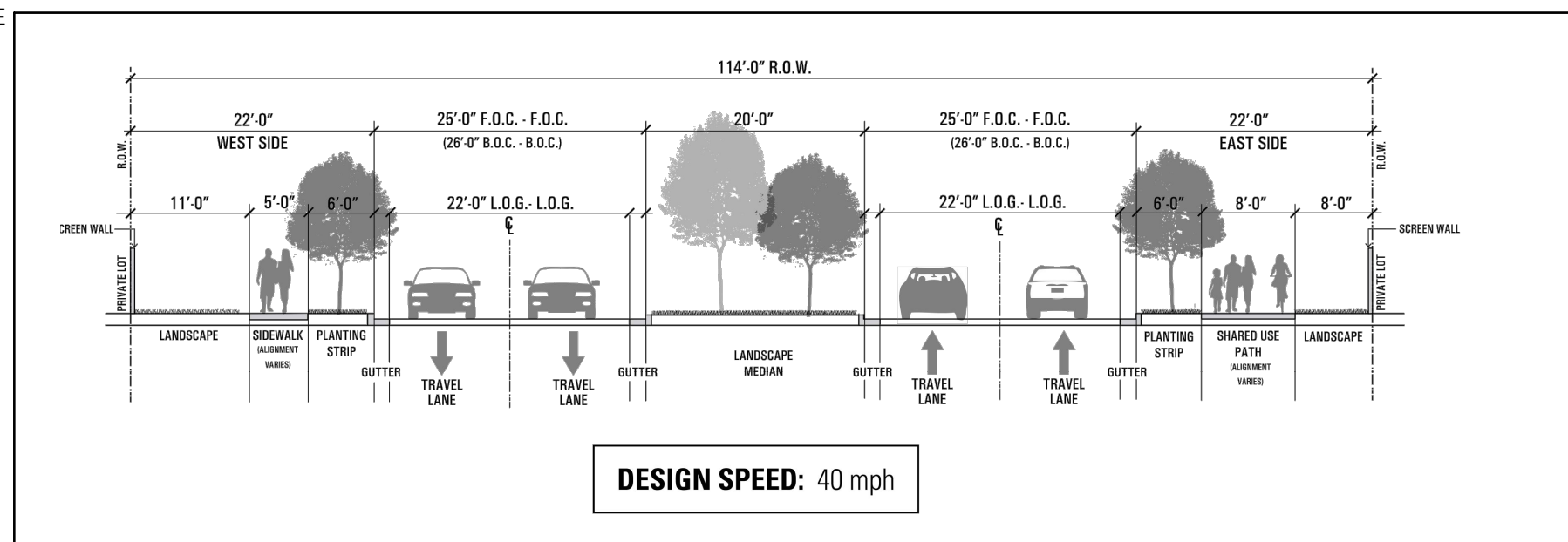
PRIMARY COLLECTOR (WITH NO SF-1 FRONTAGE)
