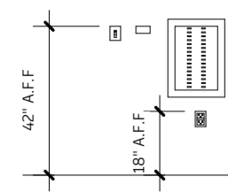
ELECTRICAL HEIGHT GUIDE 1/4" = 1'-0"
