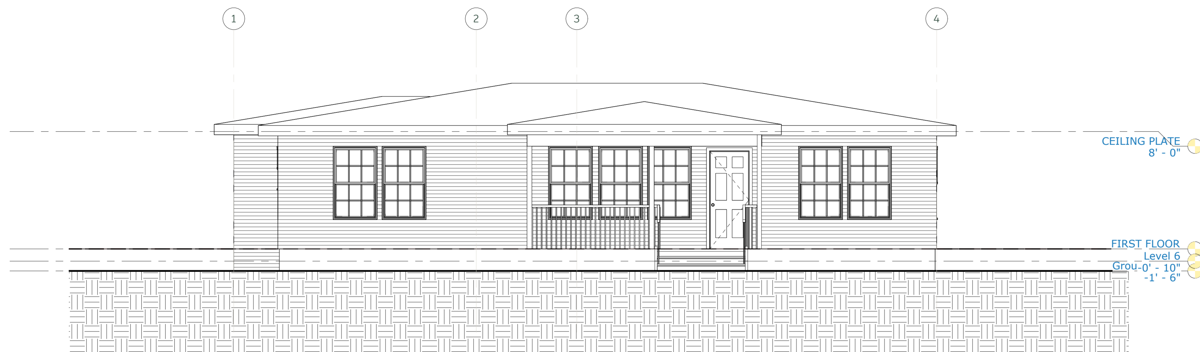
1 EXISTING NORTH ELEVATION 1/4" = 1'-0"
