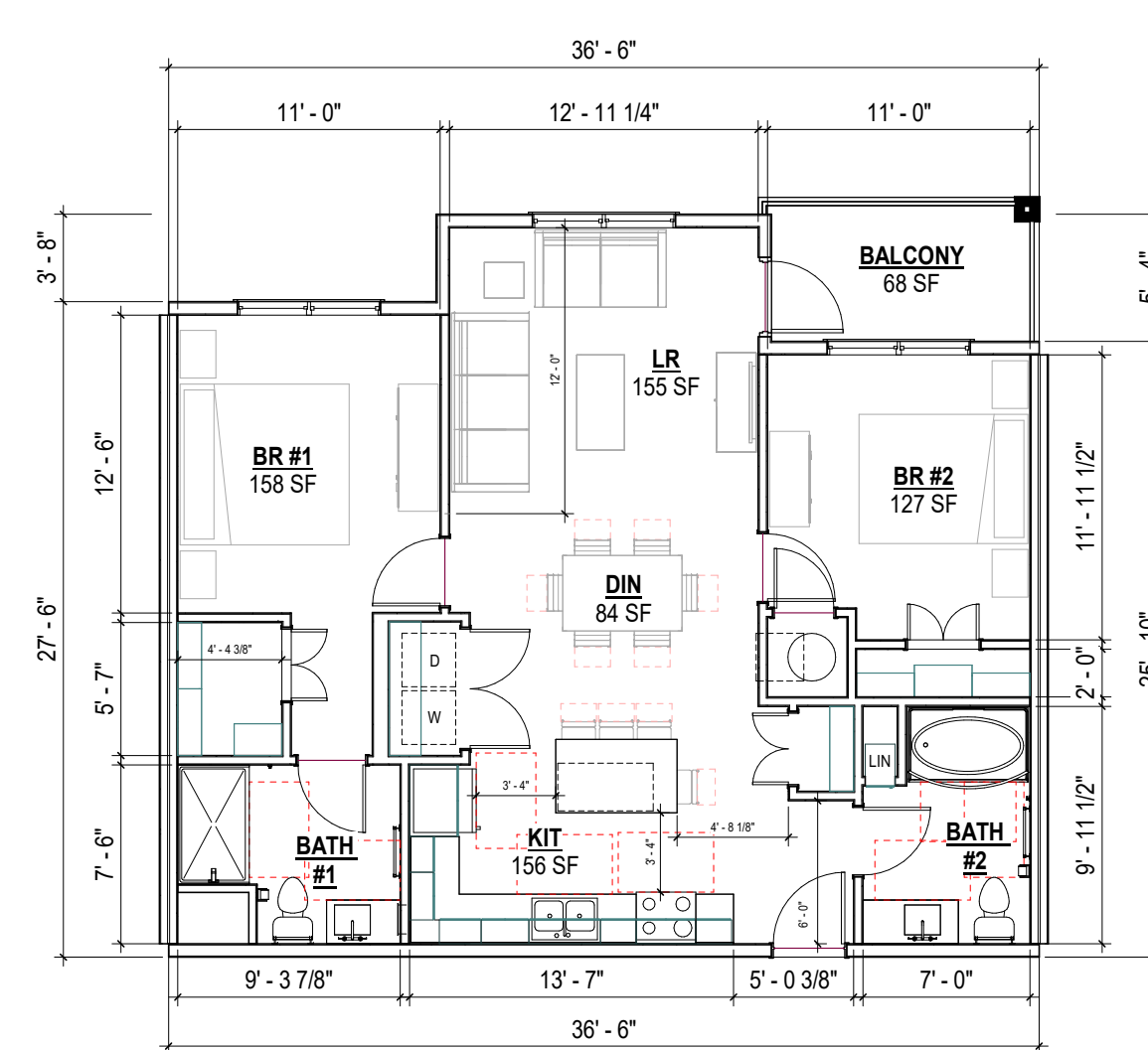
2 BR IN-LINE SPLIT
