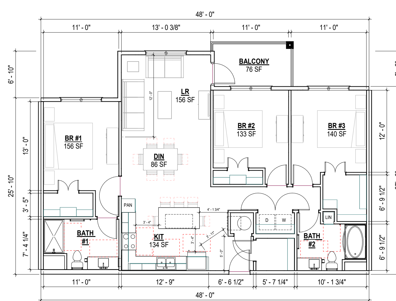
3 BR IN-LINE SPLIT
