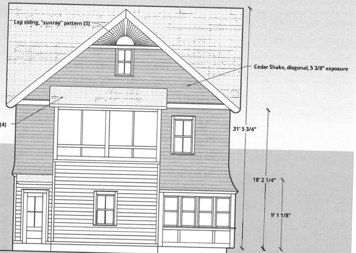
SOUTHWEST ELEVATION
