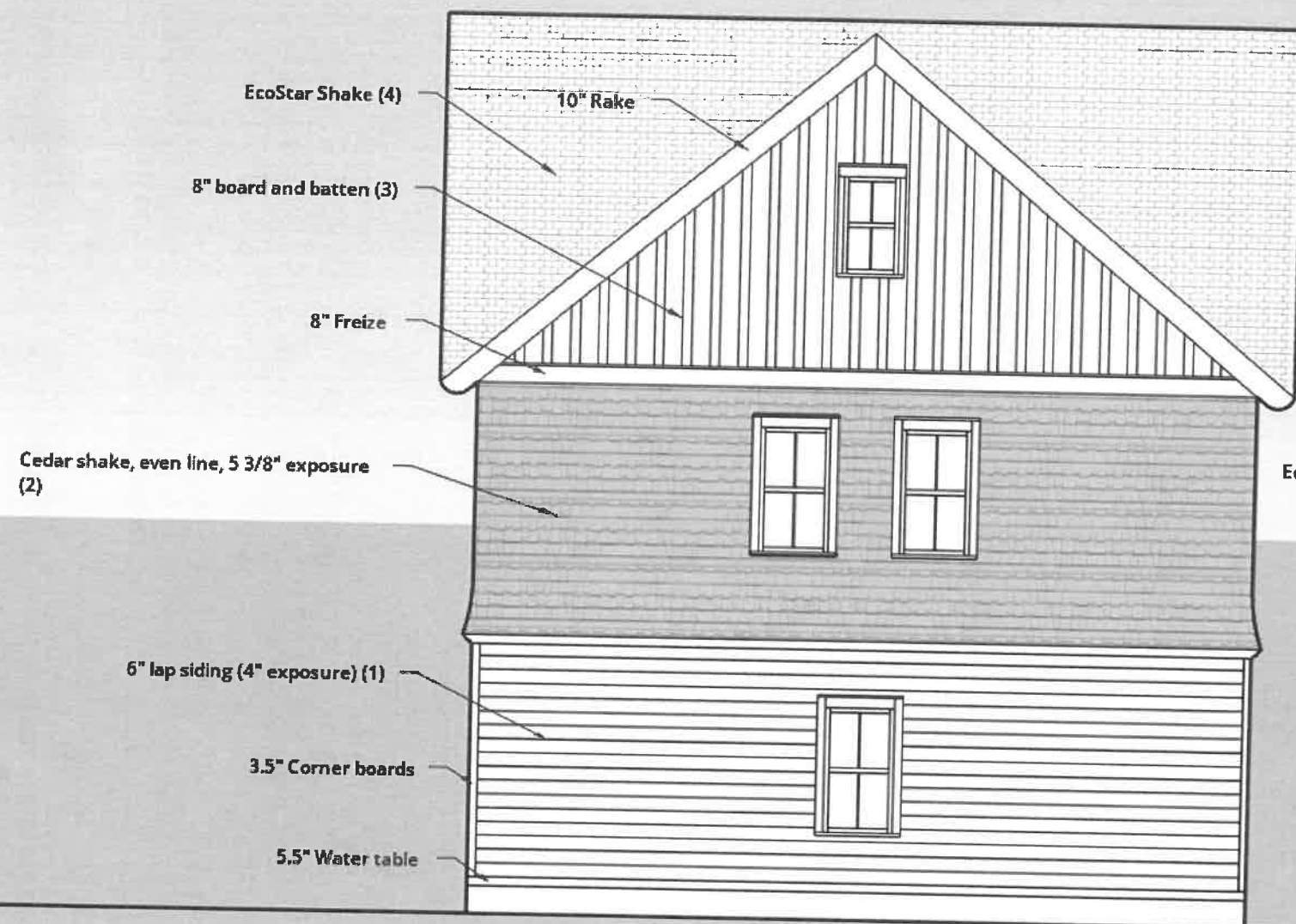
NORTHWEST ELEVATION
