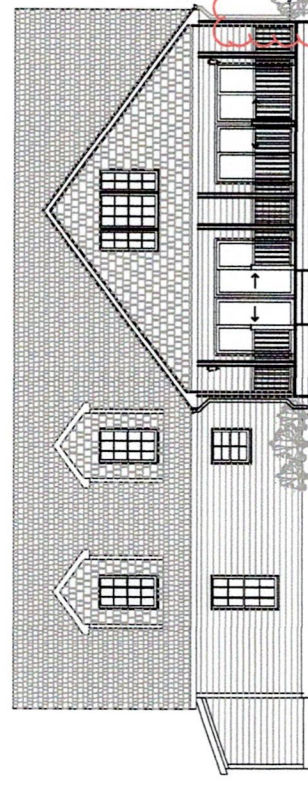
WEST ELEVATION
