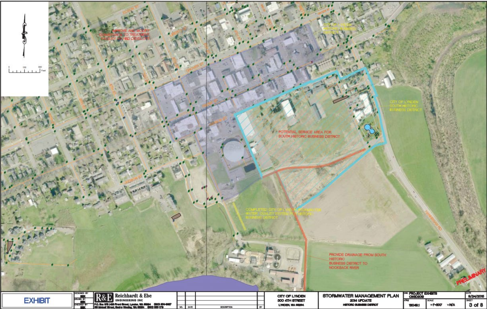
Exhibit 1: Historic Business District Sub-basin Stormwater Drainage to Facility
