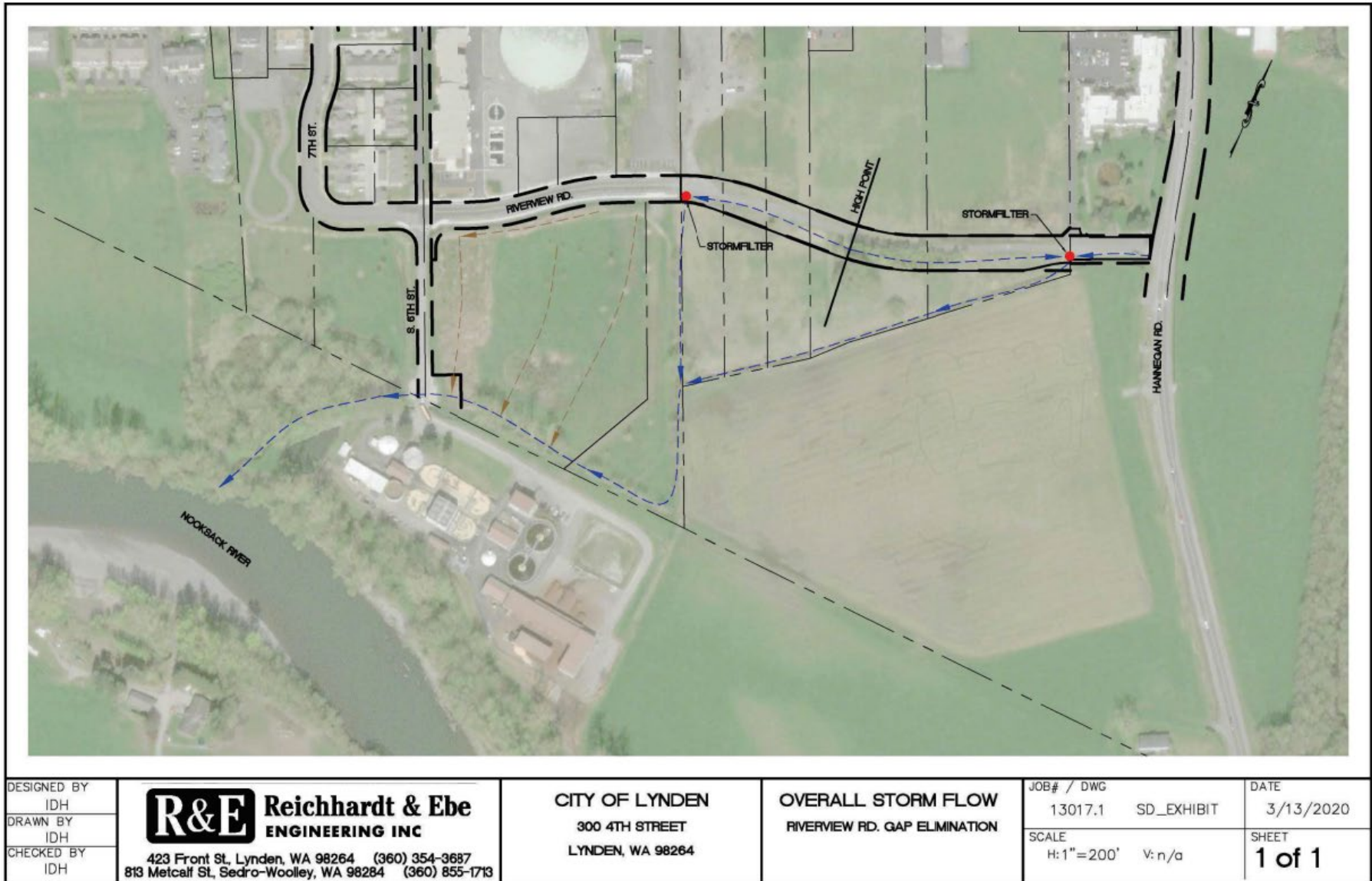
Exhibit 2: River Road Gap Elimination Stormwater Infrastructure
