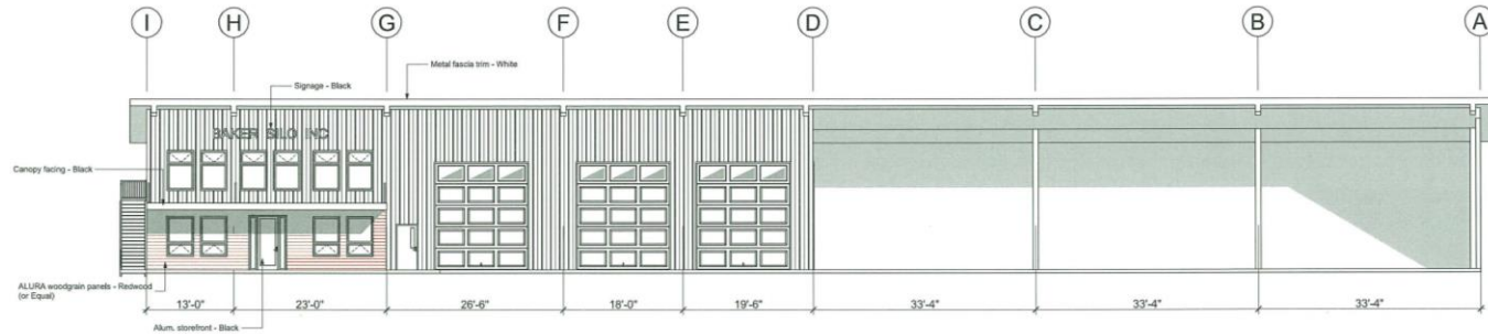
WEST ELEVATION
