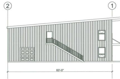
NORTH ELEVATION
