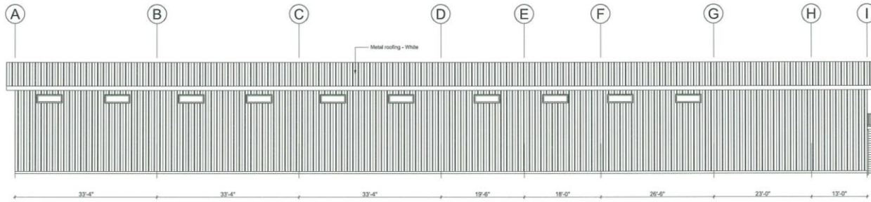
EAST ELEVATION
