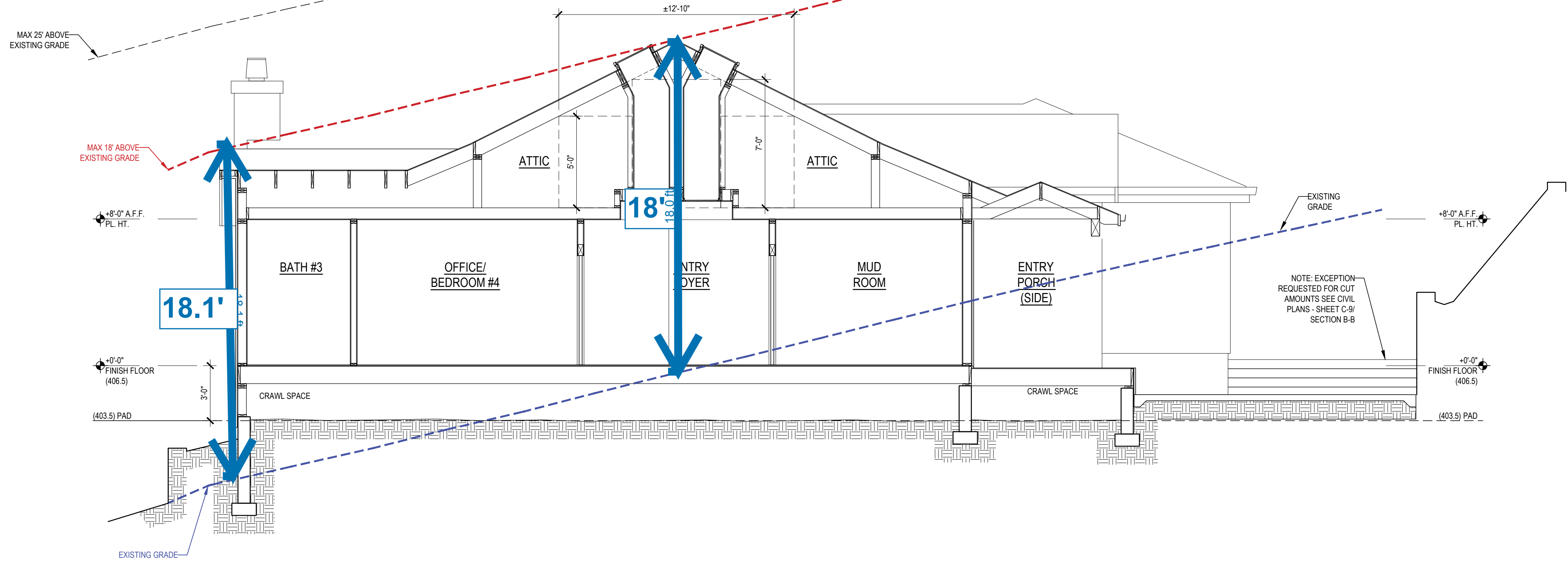
A - BUILDING SECTION
