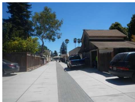
Figure 2-4 Infiltration trench, San Jose (Source: City of San Jose)
