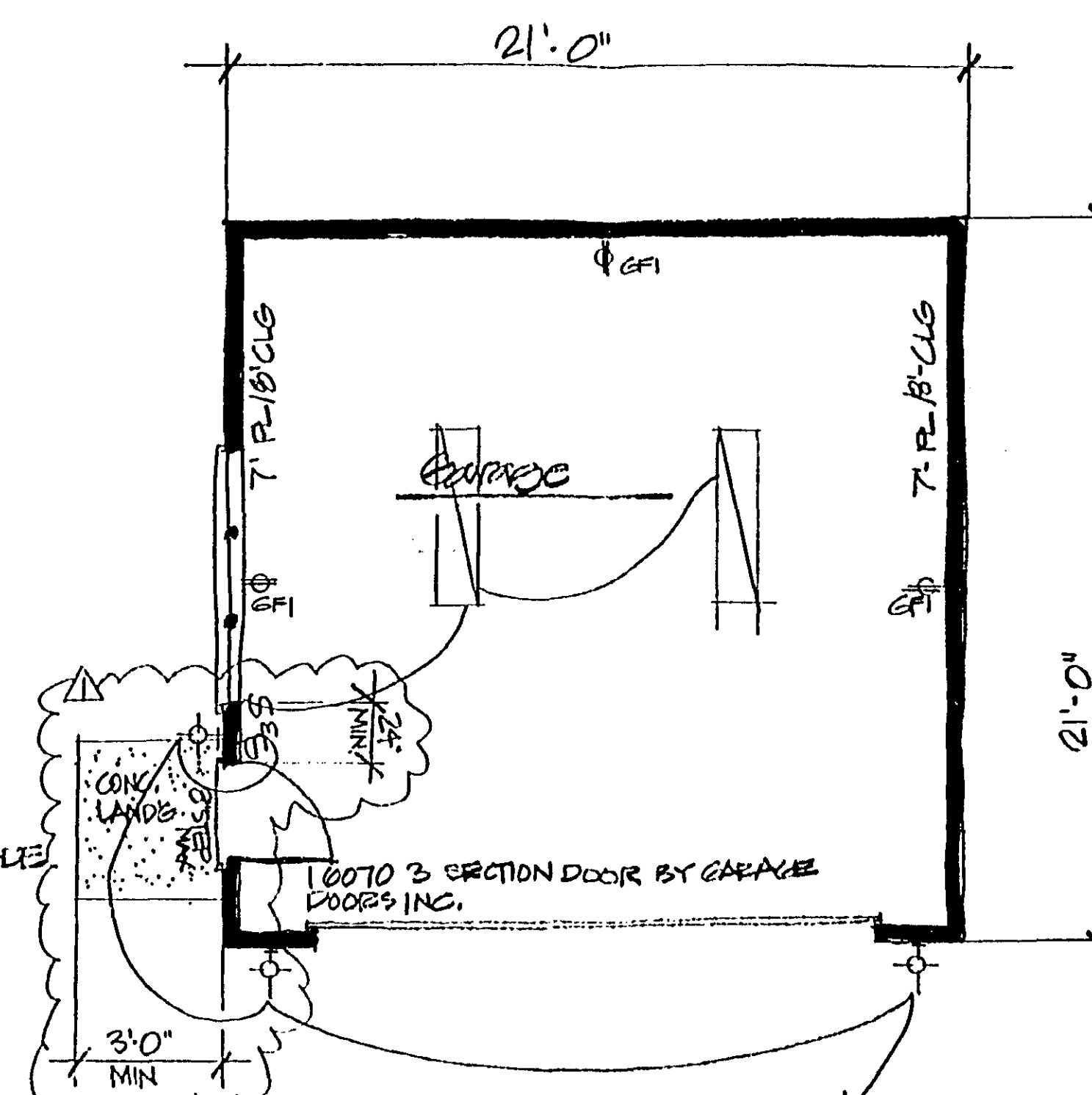
GARAGE PLAN
