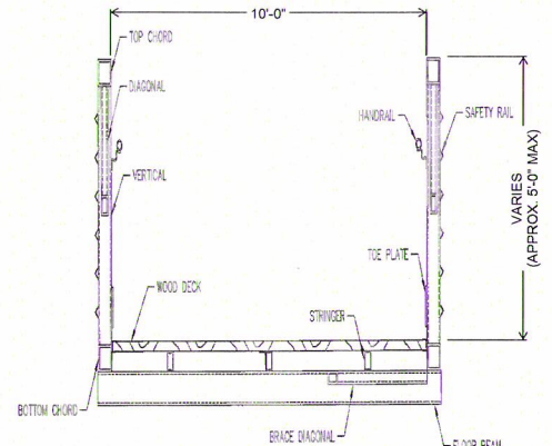
TYPICAL SECTION (TIMBER DECK) NOT TO SCALE
