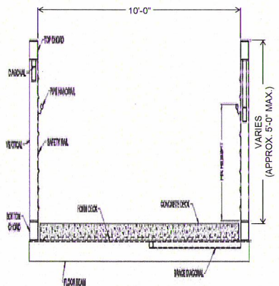
TYPICAL SECTION (CONCRETE DECK) NOT TO SCALE
