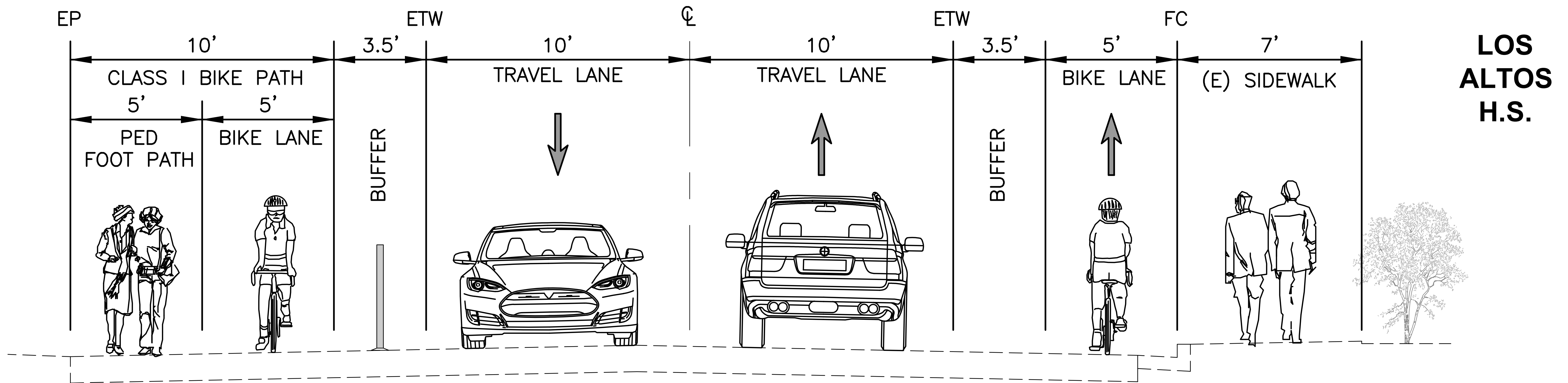
CONCEPT 3 JARDIN DRIVE PROPOSED CROSS SECTION - FACING EAST (PANCHITA WAY TO CASITA WAY)
