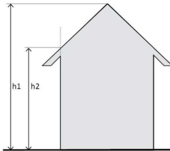
Figure 18.45.070-1. Where allowed by LFPMC 18.45.070, the height of a building with a pitched roof is (h1 + h2)/2 , where h2 is measured at the surface of the roof where it intersects with a projection of the outside edge of the building wall. Where the wall/roof configuration varies, the building height shall be at the point where the height is the maximum.
