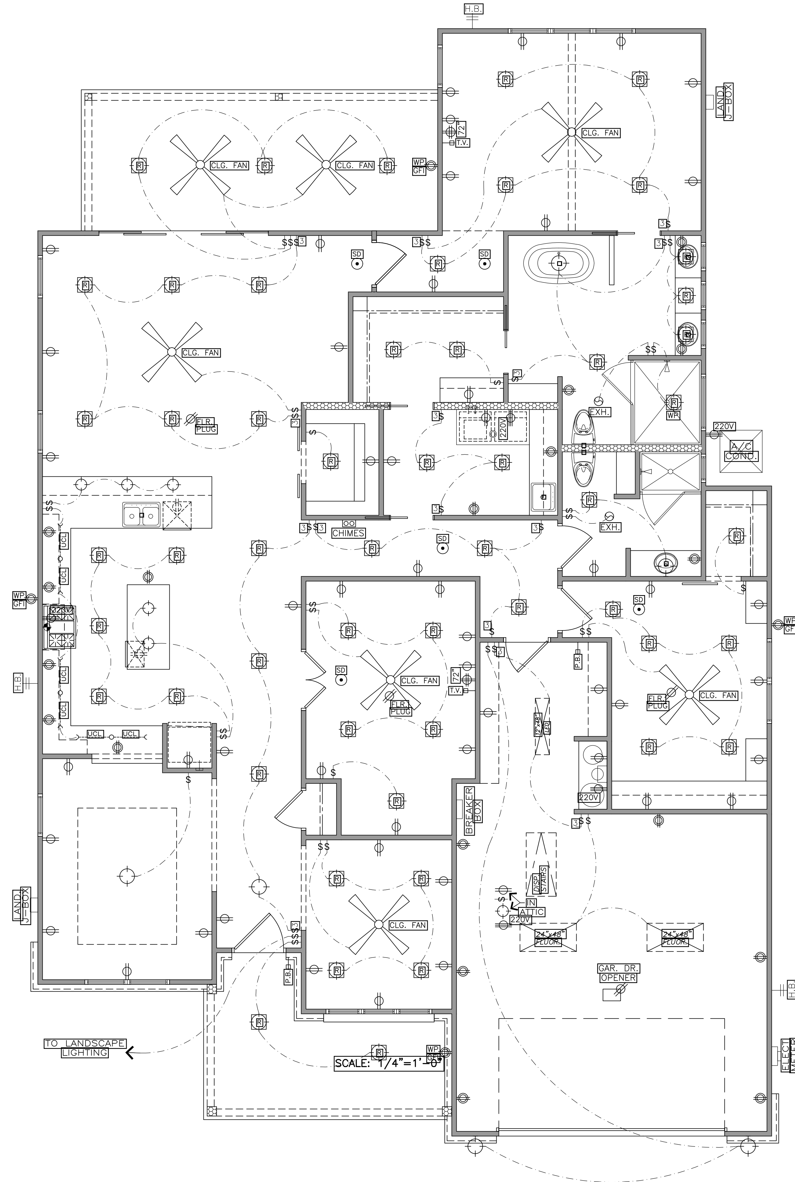
MAIN FLOOR ELECTRICAL PLAN
