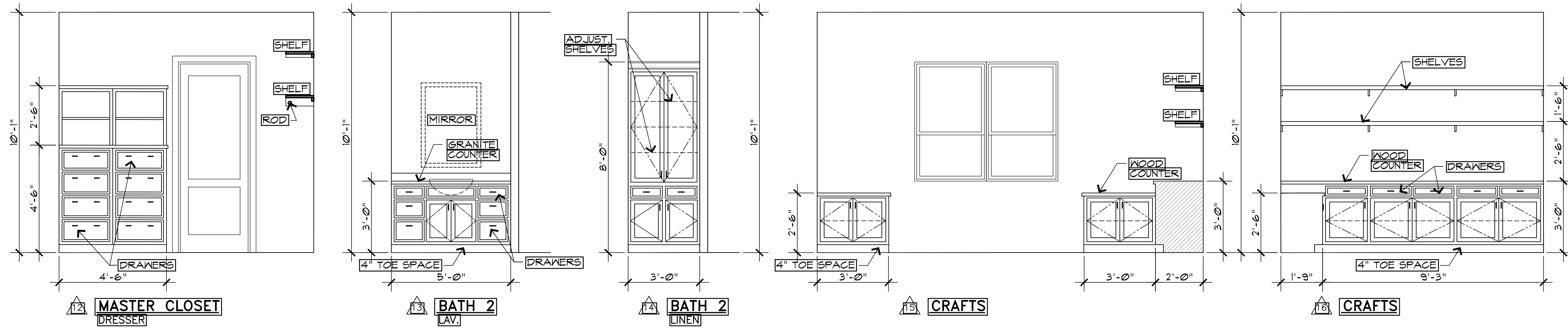
INTERIOR ELEVATIONS SCALE: 3/8"=1'-0"
