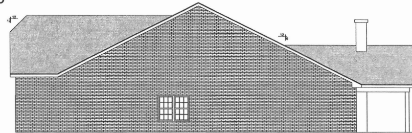
RIGHT ELEVATION 1/8"---1'-0"
