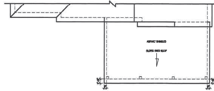
B 1 ROOF PLAN SCALE: 1/8" = 1'-0"
