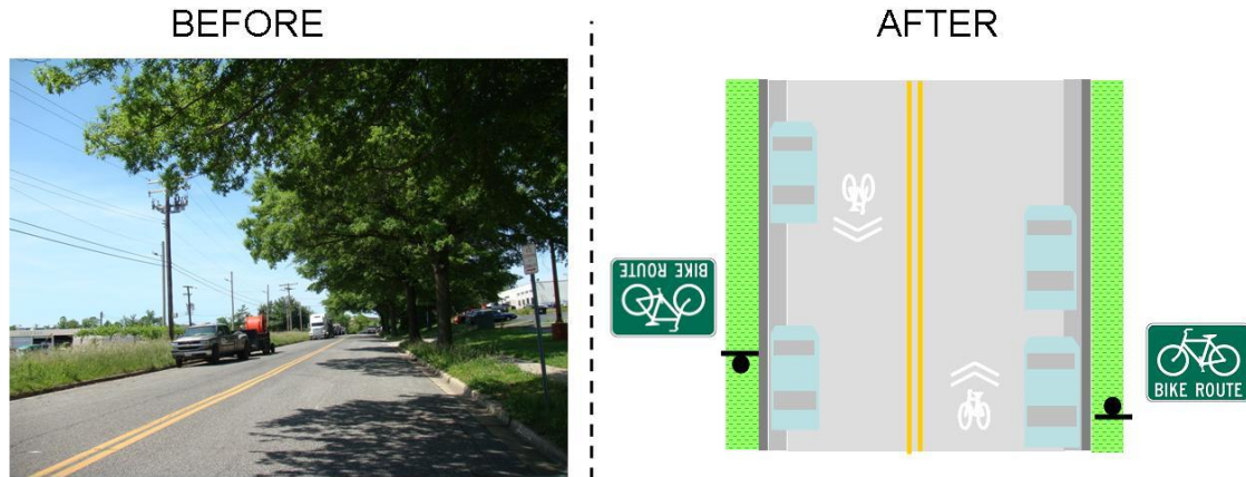
Figure 22: Before and After Signage/Striping Improvements for Staggers Lane
