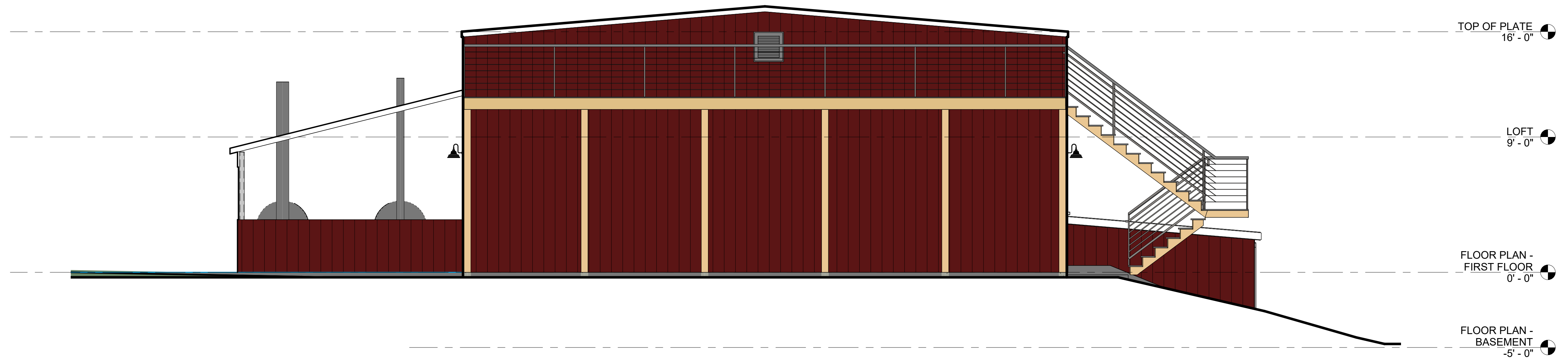
② Elevation - North 1/4" = 1'-0"
