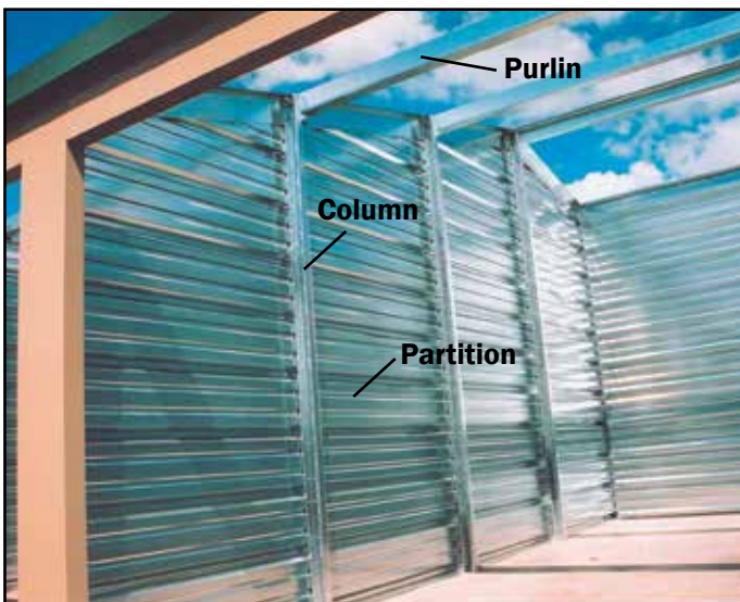
b. The interior structure features pre-punched columns and purlins for bolt together connections to simplify installation. The entire structure is zinc coated to inhibit rust. A 3":12" pitch building is shown above.
