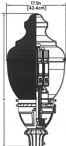
RL34BANNxxW configuration shown
