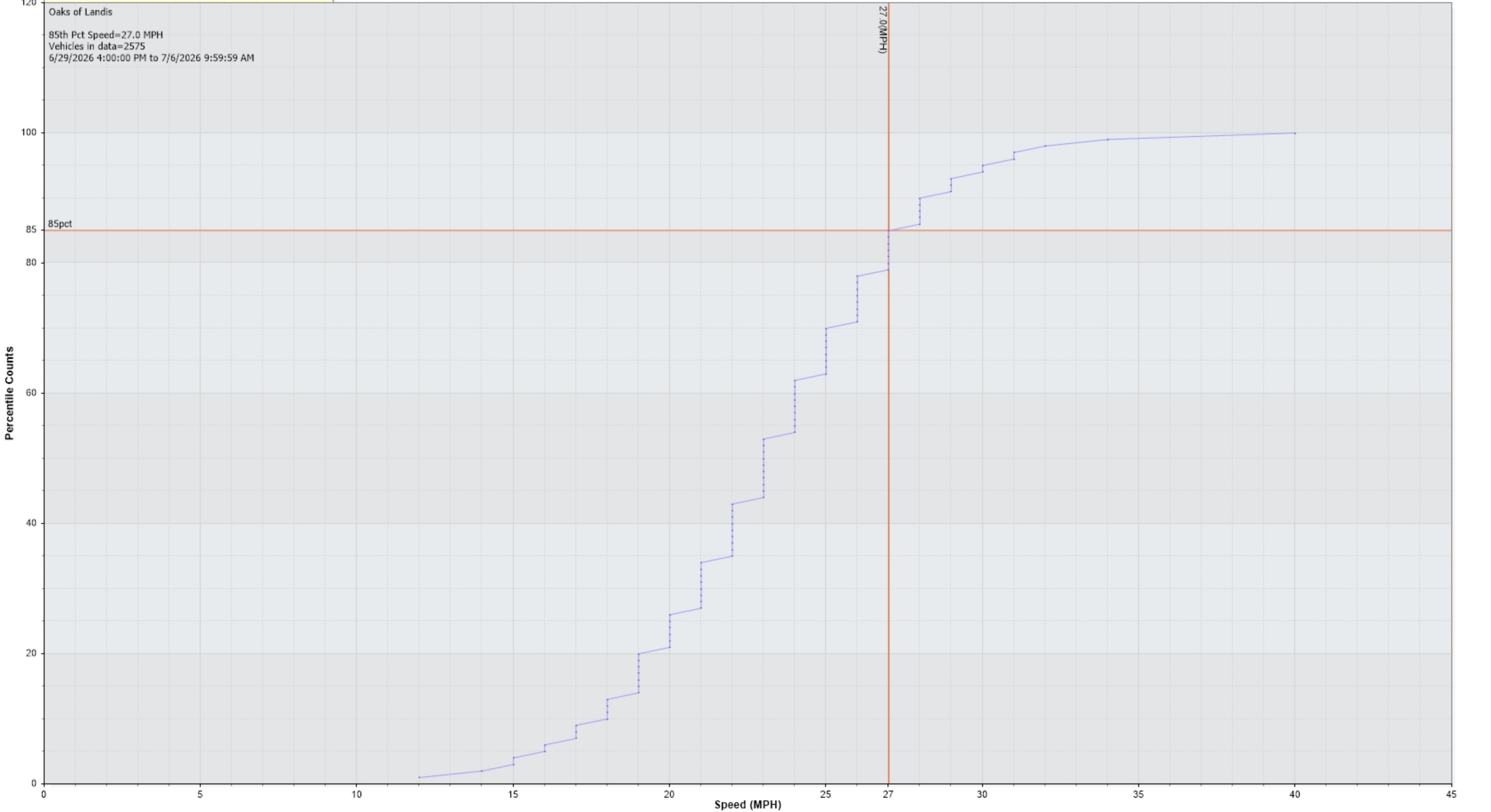
Percentile Counts Vs. Speed for [Oaks of Landis: Merged]
