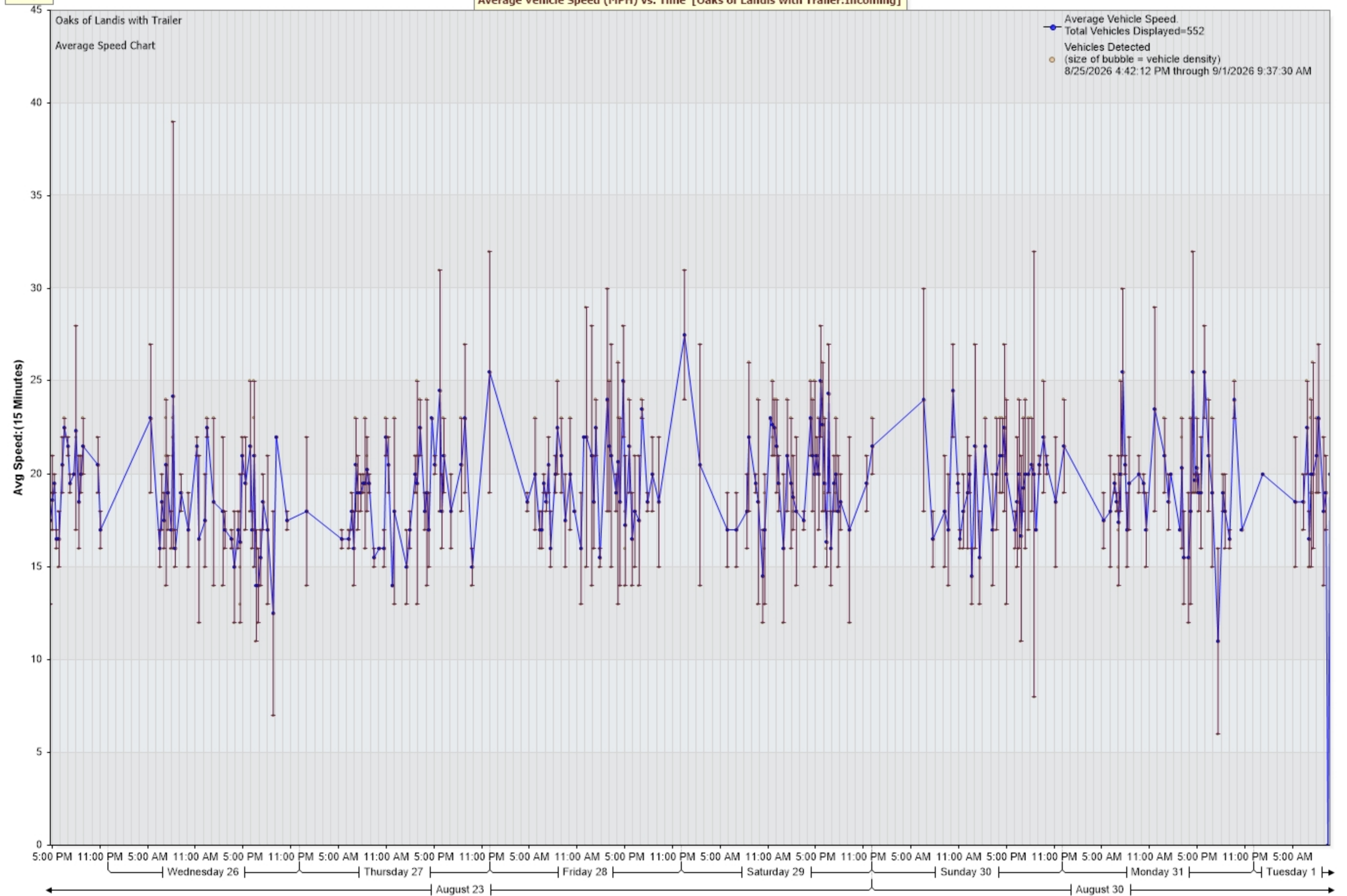
Average Vehicle Speed (MPH) vs. Time [Oaks of Landis with Trailer:Incoming]
