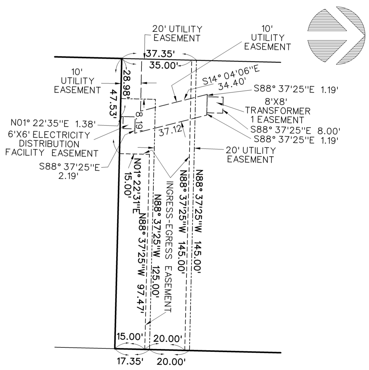
DETAIL 1"=30'
