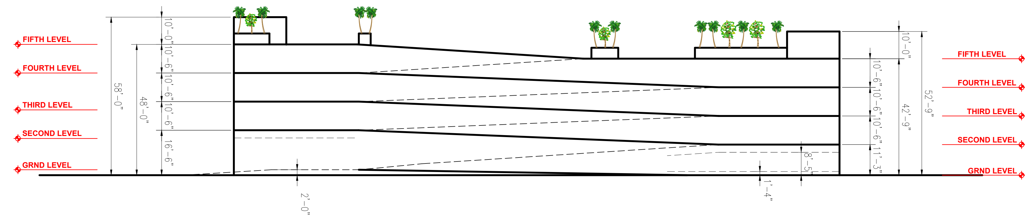
SECTION DIAGRAM
