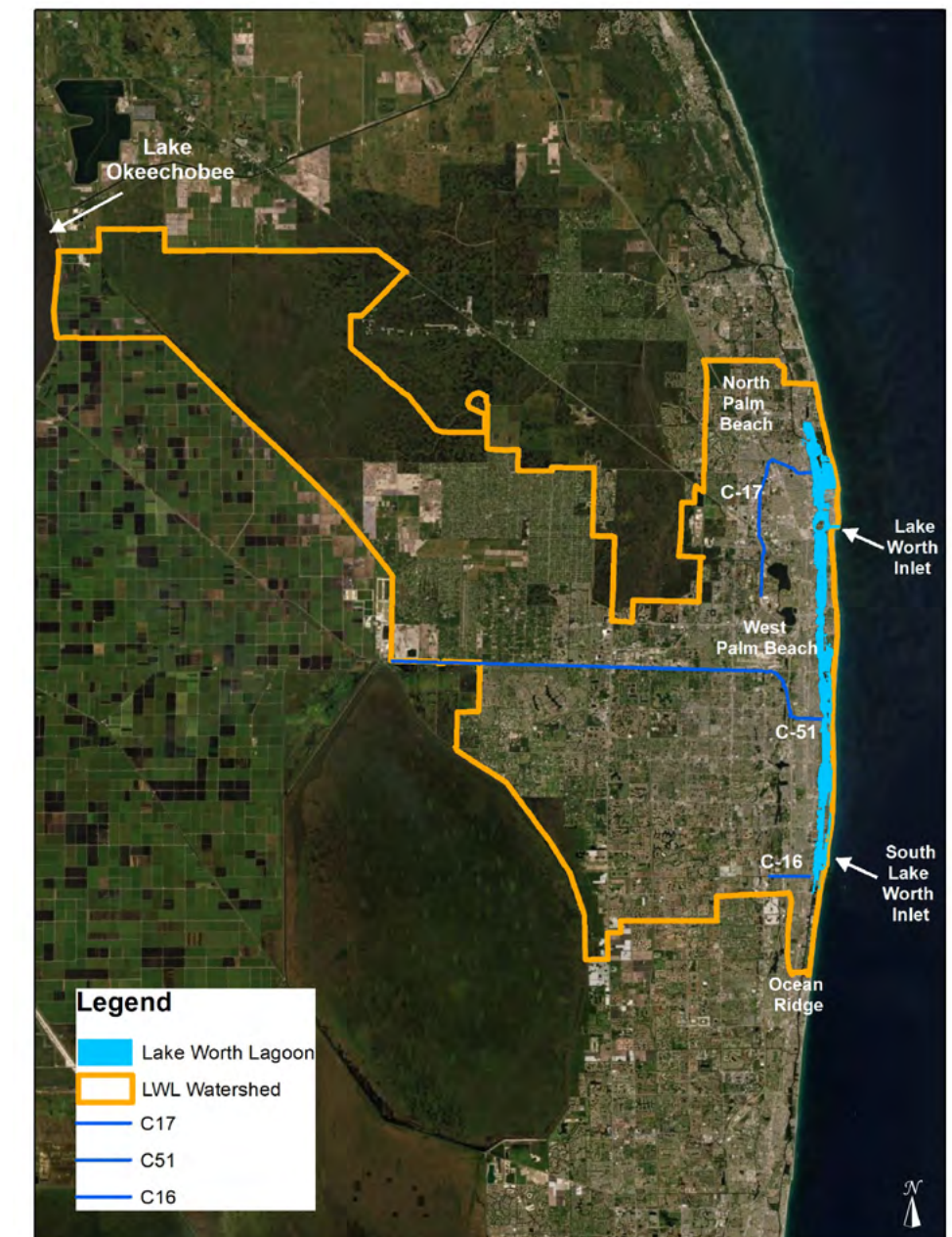
FIGURE 1.1 WATERSHED MAP
