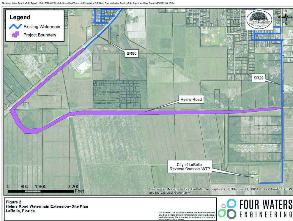
Figure 2: Site Plan
