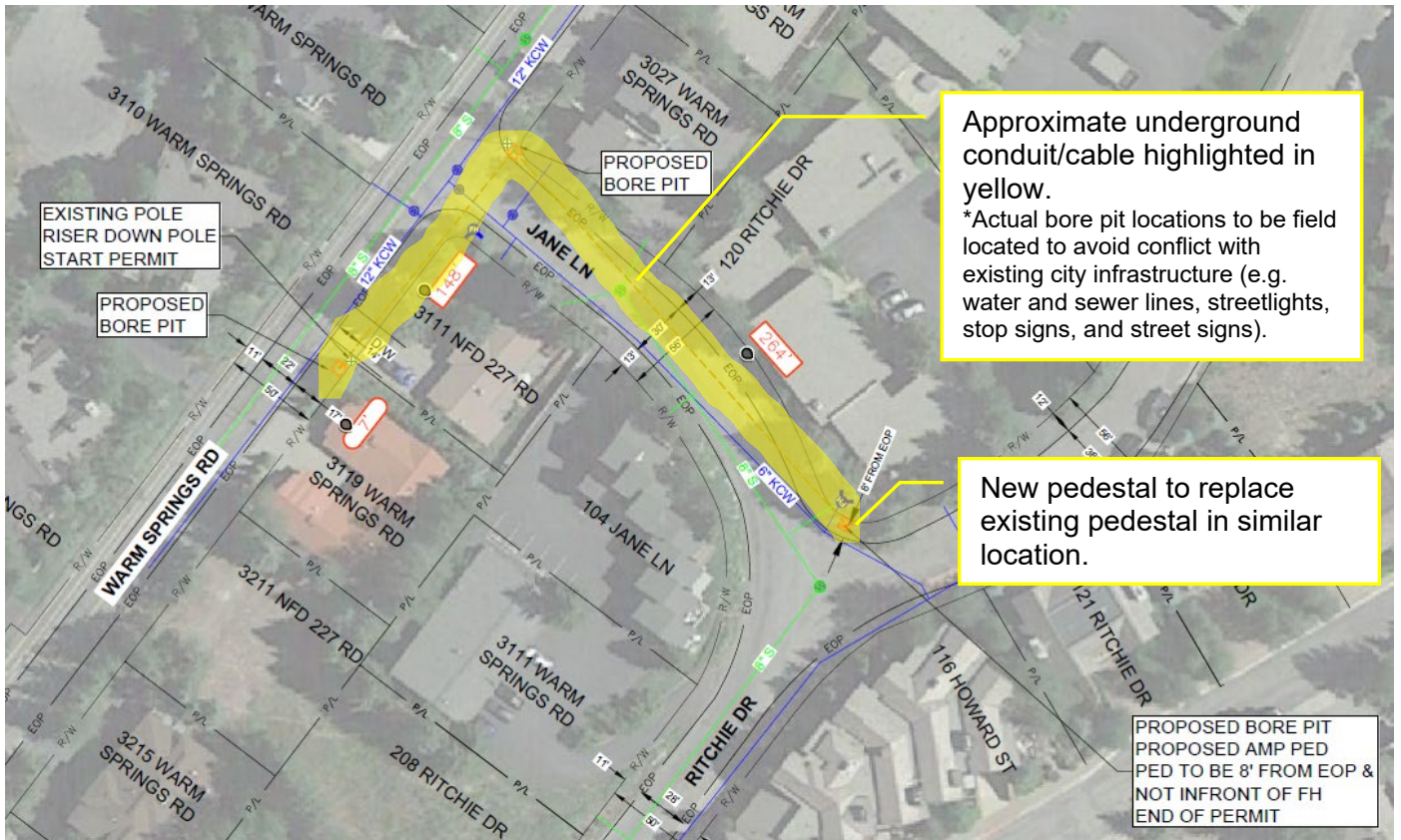
BASE FIGURE PROVIDED BY COX COMMUNICATION ANNOTATED BY CITY ENGINEER ROBYN MATTISON (YELLOW TEXT BOXES) TO CLARIFY IMPROVEMENTS INCLUDED IN RIGHT-OF-WAY AGREEMENT NO. 24935
