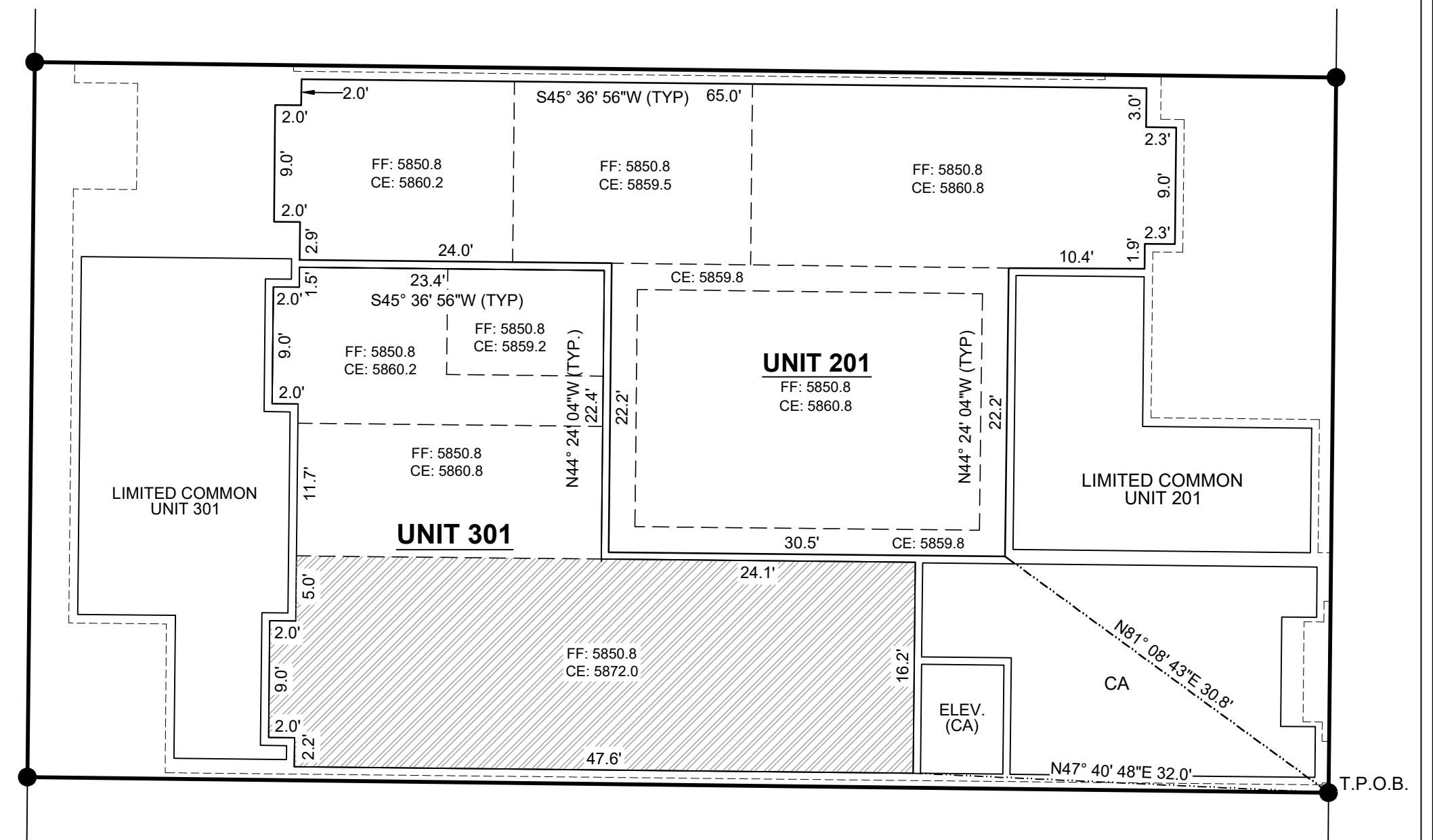
SECOND FLOOR
