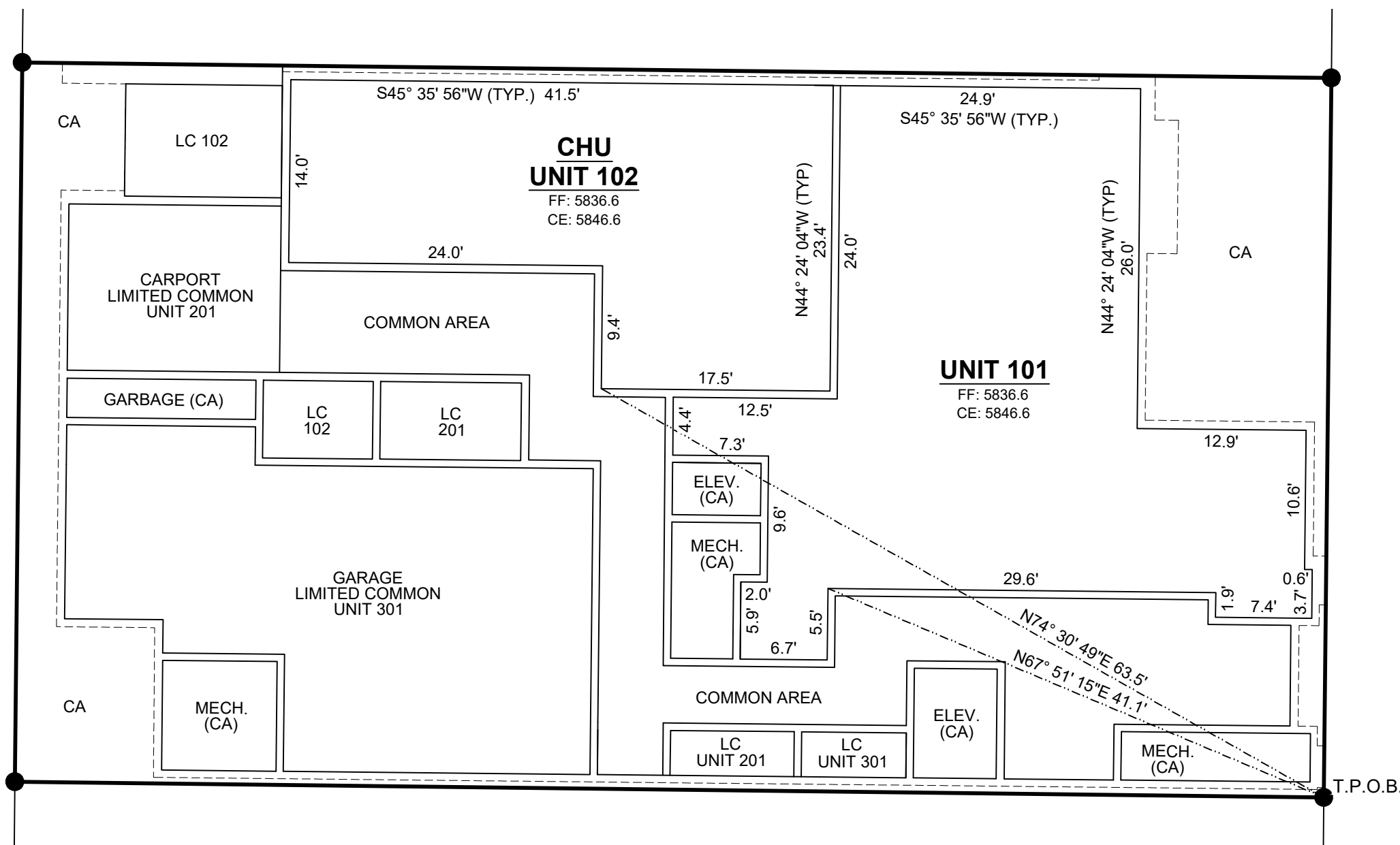
FIRST FLOOR
