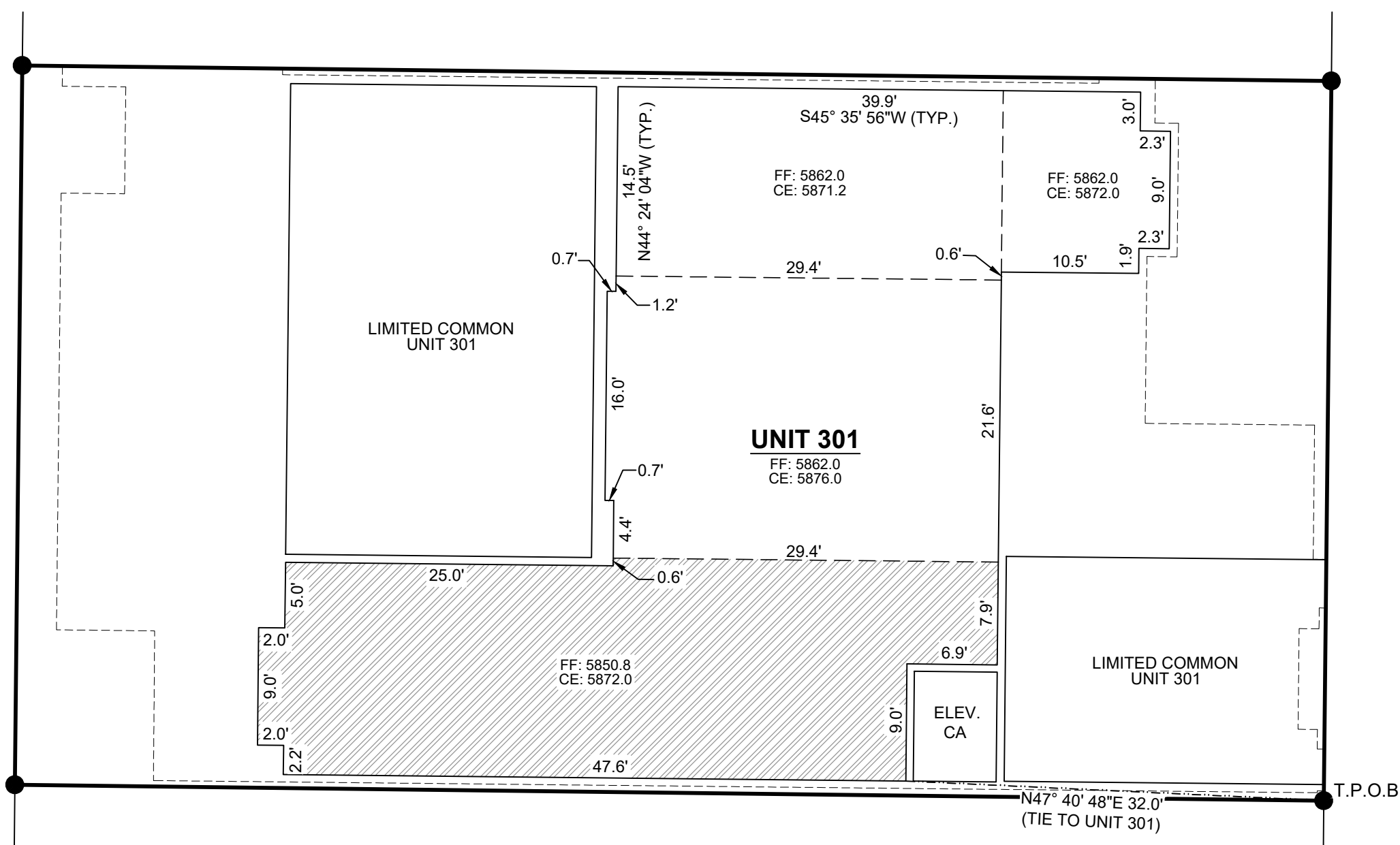
THIRD FLOOR
