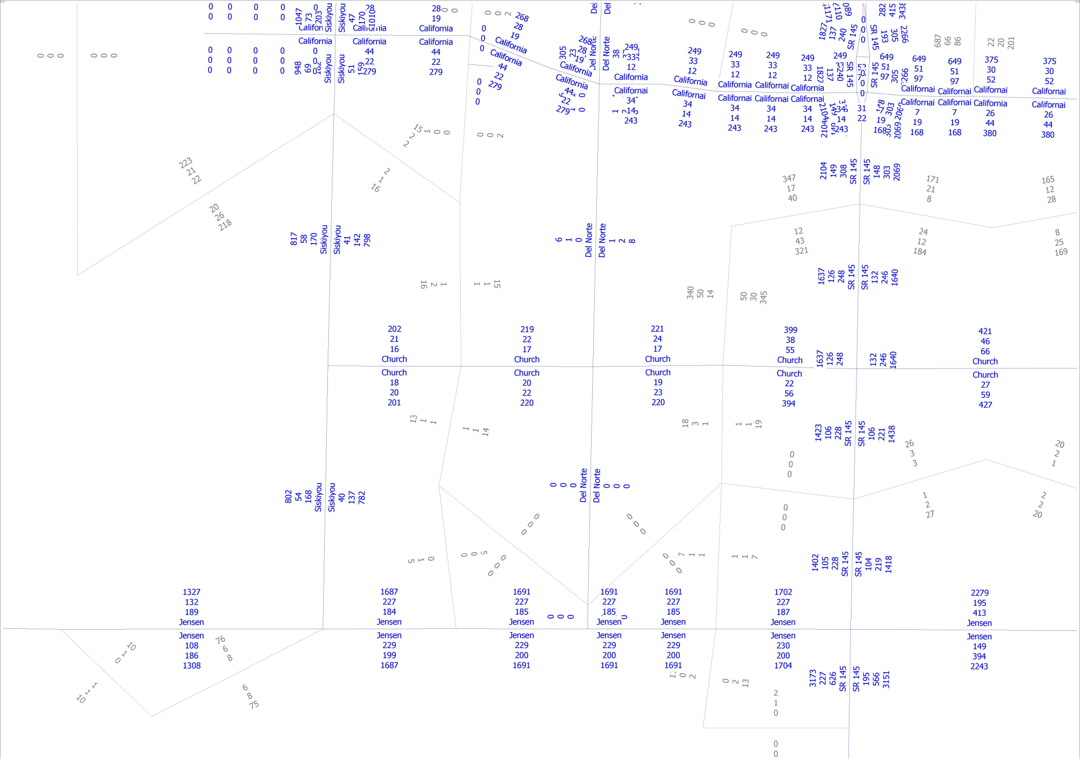
Crown-Schaad TIA Base Year 2019 AM, PM and Daily Volume
