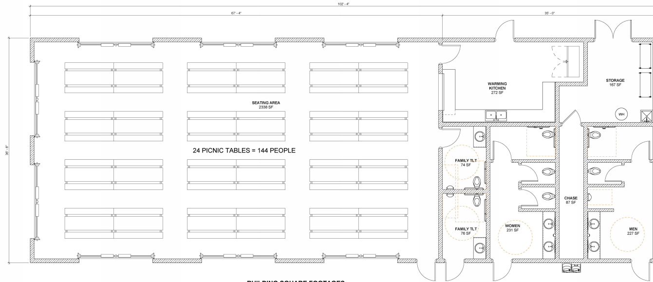
FIRST FLOOR PLAN - CONCEPT B
