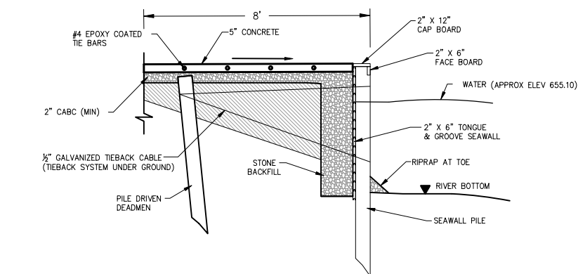
TYPICAL SEAWALL SECTION
