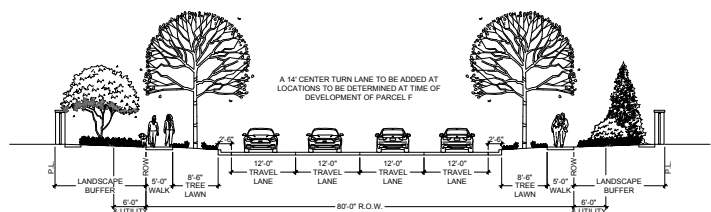
COLLECTOR A W/OUT CENTER TURN LANE
