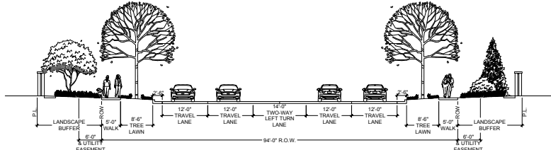
COLLECTOR A W/CENTER TURN LANE
