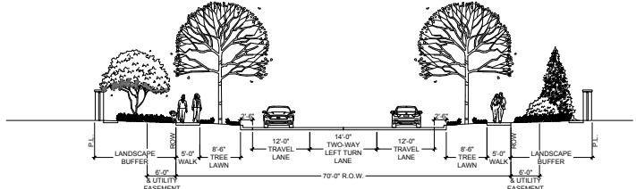
COLLECTOR C W/CENTER TURN LANE
