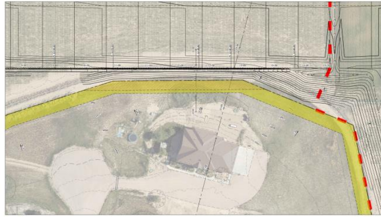
GRADING WITH MINIMAL OFFSITE GRADING IMPACT (WALLS)
