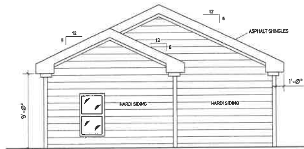
REAR ELEVATION
