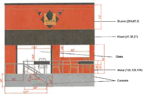
BACK ELEVATION
