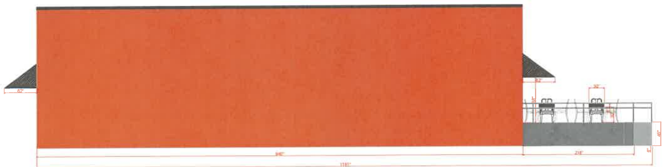
LEFT ELEVATION
