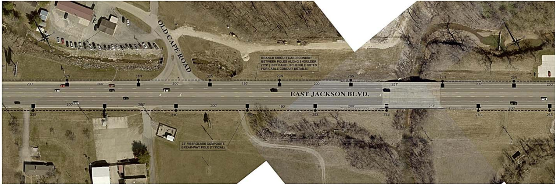
2 ROADWAY LIGHTING LAYOUT - SECTION 4 E1.2 SCALE: 1" = 50'
