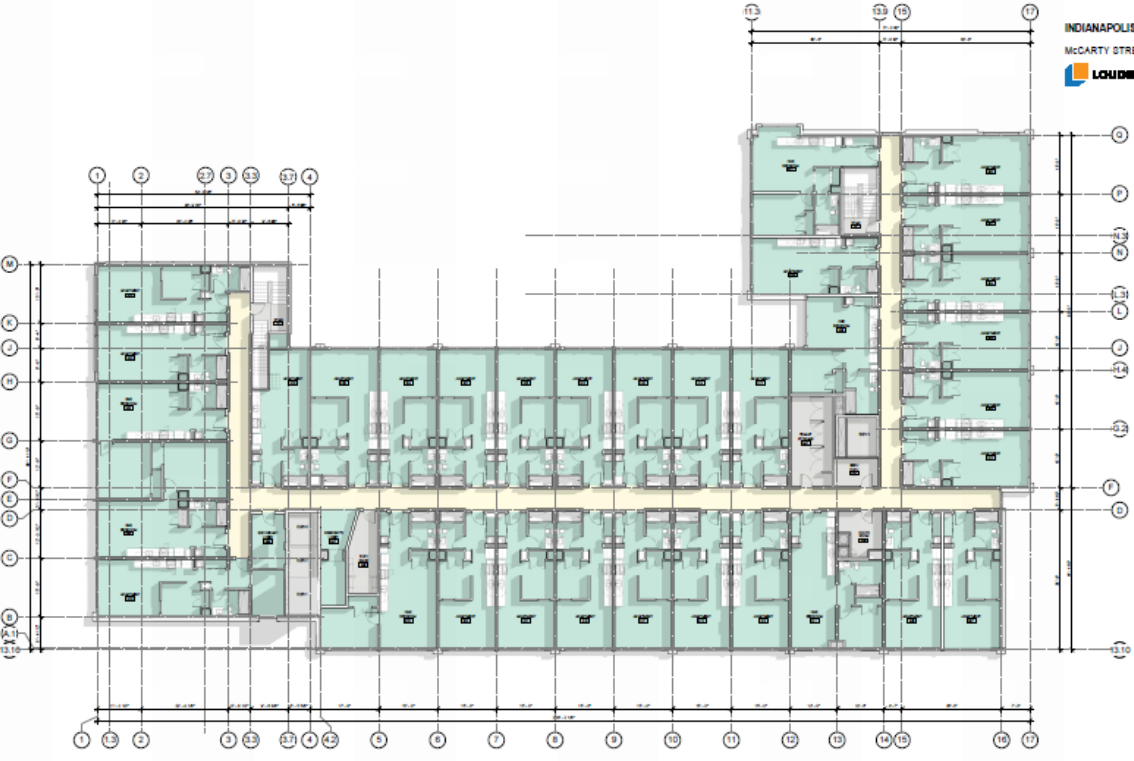
SIXTH FLOOR PLAN DATE: 10/27/2011 11:11 AM
