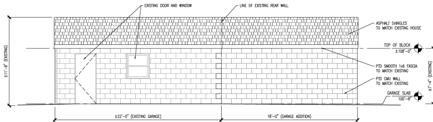
3 North Exterior Elevation 1/4"=1'-0" 0 2' 4' 8'
