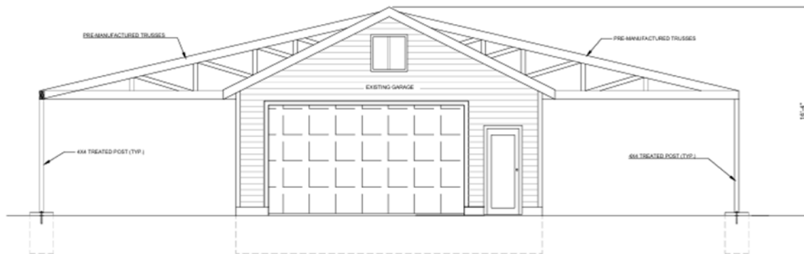
2 SOUTH ELEVATION 3/4" = 1'-0"
