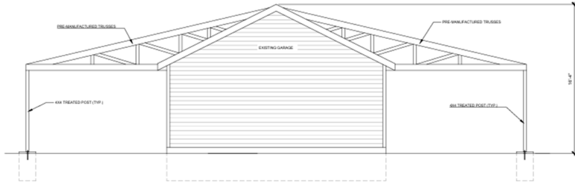
1 NORTH ELEVATION 3/4" = 1'-0"
