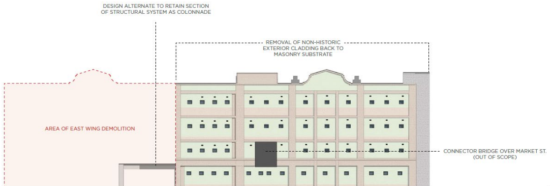
EXISTING NORTH ELEVATION (POST DEMOLITION) NOT TO SCALE
