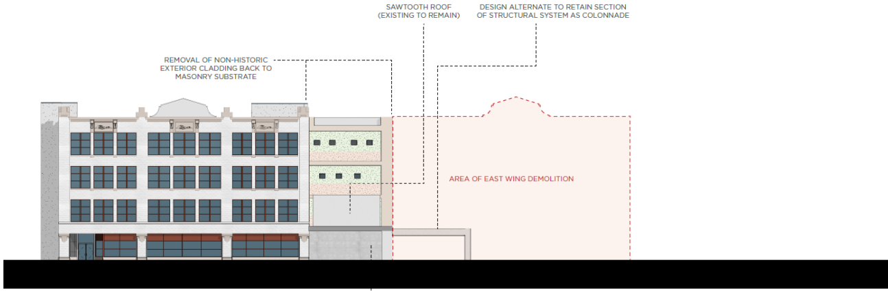
EXISTING SOUTH ELEVATION (POST DEMOLITION) NOT TO SCALE
