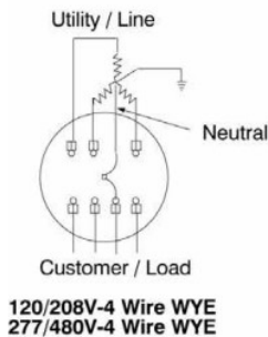
Figure 5 Typical Three-phase Service Connection (Meter Base Front View)
