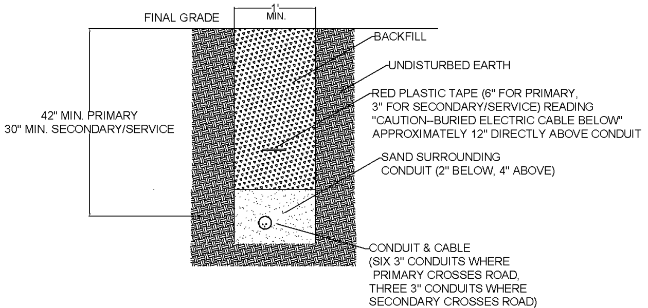
TRENCH DETAIL
