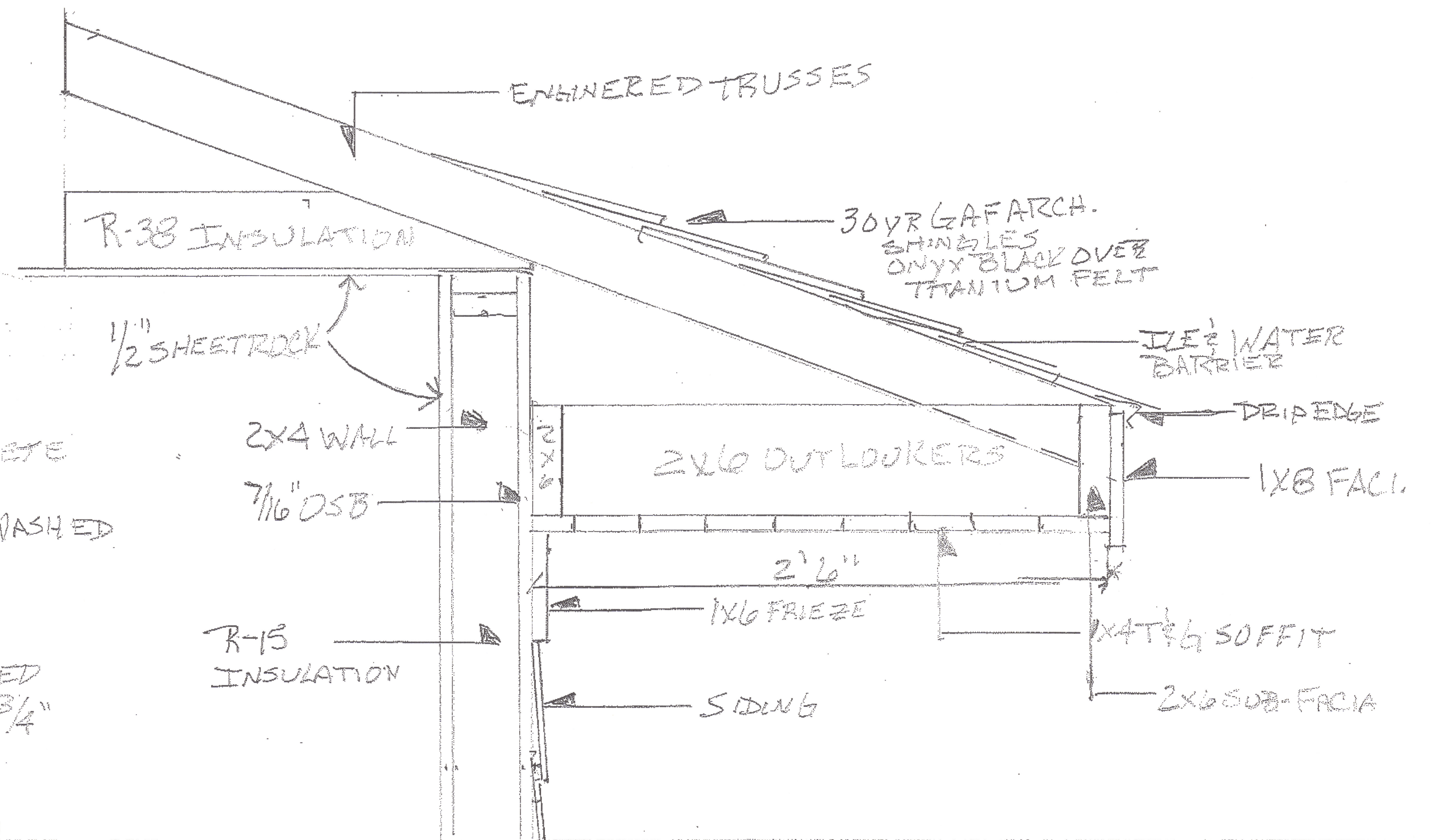
SOFFIT DETAIL 1 1/2" = 1'
